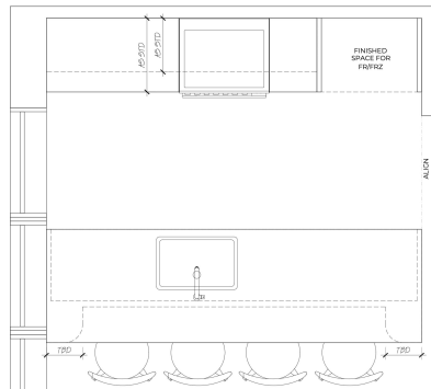
Key Plan: Kitchen
